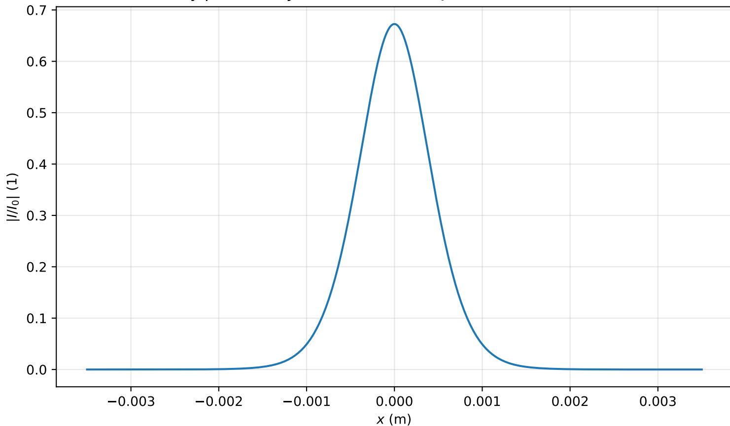
Intensity profile I(x, y = 0, z = 2.548m)/I_0 , \text{Pin}=0.5\text{Pcr} , artificial time
